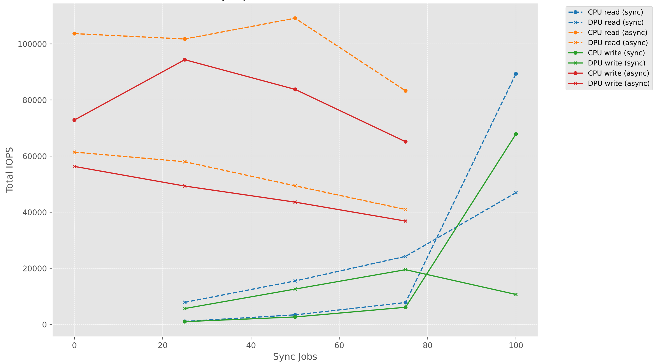
IOPS vs Sync Jobs (mixed) - SEQ (CPU vs DPU)
